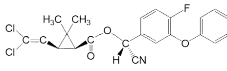
【D】 (1 S -3 S - \alpha R ) ( R )-Cyano (4-fluoro-3- phenoxyphenyl)methyl (1 S , 3 S )-3- (2, 2-dichlorovinyl)-2, 2- dimethylcyclopropane-1-carboxylate
