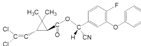
【H】 (1 S -3 R - \alpha R ) ( R )-Cyano (4-fluoro-3- phenoxyphenyl)methyl (1 S , 3 R )-3- (2, 2-dichlorovinyl)-2, 2- dimethylcyclopropane-1-carboxylate
